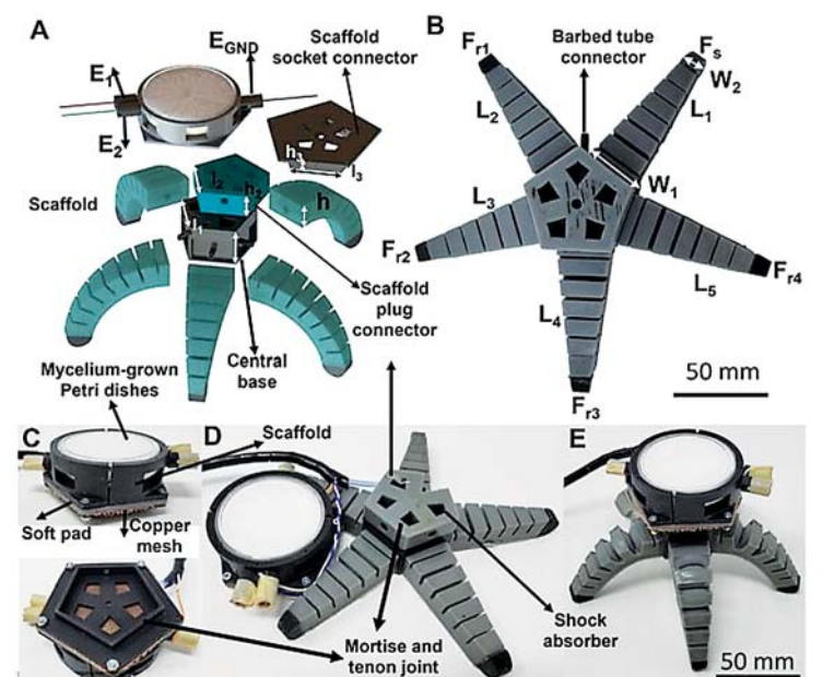
A specialised housing containing a mycelium sample is built into a soft robot to act as the walking device's brain.
